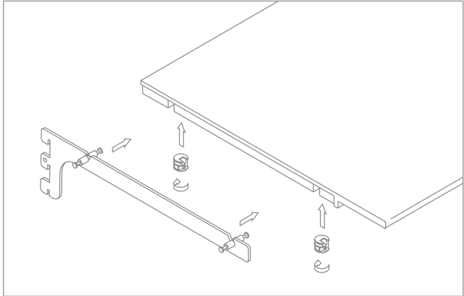
Typical fixing detail
